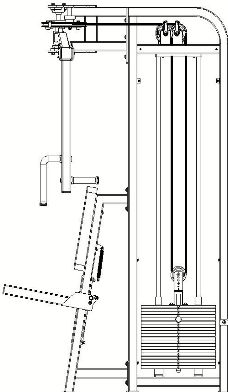
Wire rope routing diagram
